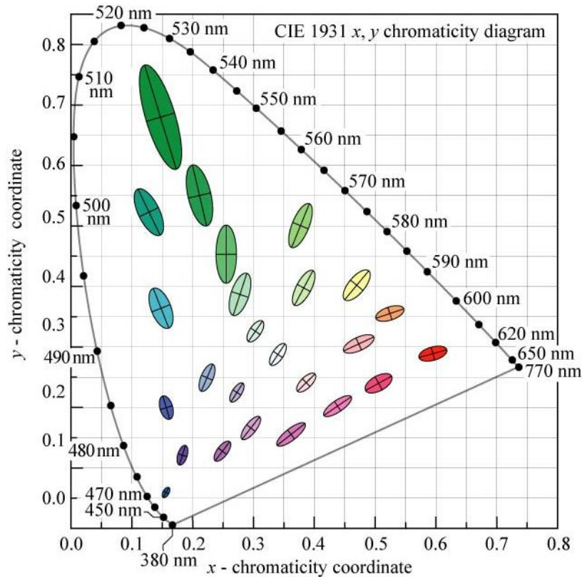
Figure 9: MacAdam ellipses
